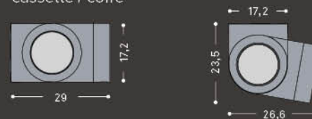
cassette / cofre
